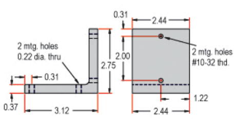
2.62" Z-Axis Adapter Plate (#54-378)
