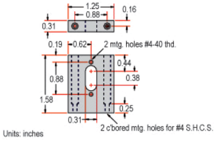
1.25" Z-Axis Adapter Plate (#54-368)
