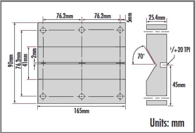
V-Block Base
