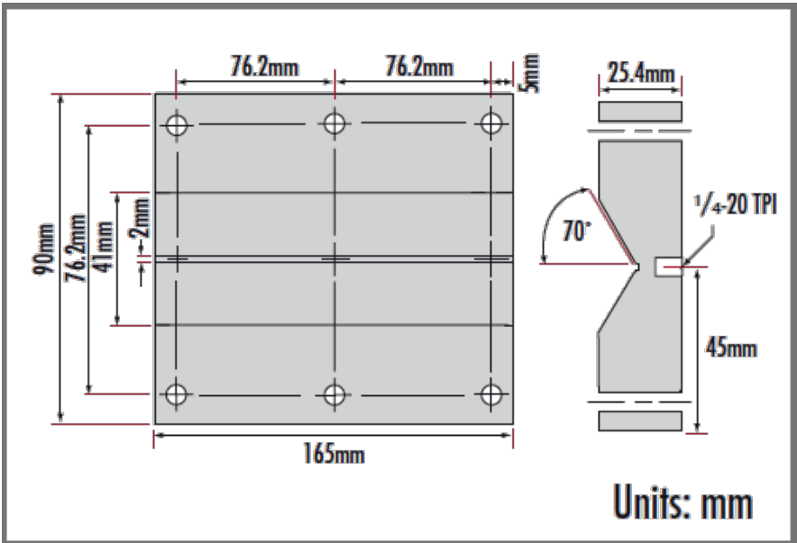
V-Block Base
