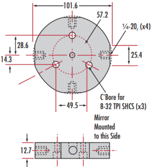
Mounting Plate for 76.2mm Mirrors, #63-375
