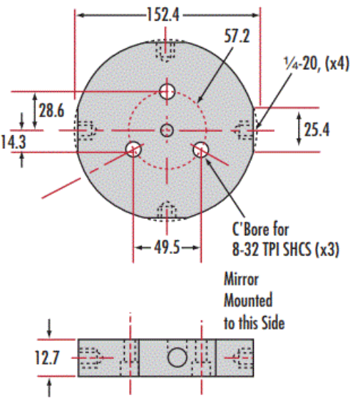
Mounting Plate for 101.6mm Mirrors, #83-977
