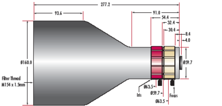
0.08X & 0.06X Telecentric Lens Units: mm
