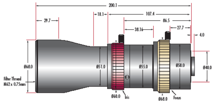
1X & 0.73X Telecentric Lenses Units: mm
