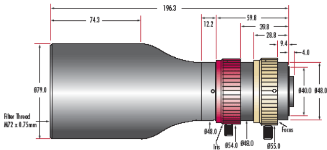
0.25X & 0.18X Telecentric Lenses Units: mm
