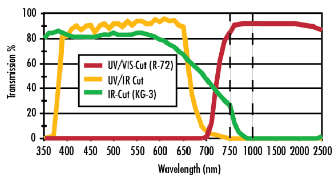
Infrared Filters
