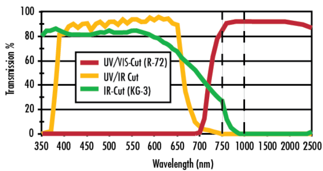
Infrared Filters
