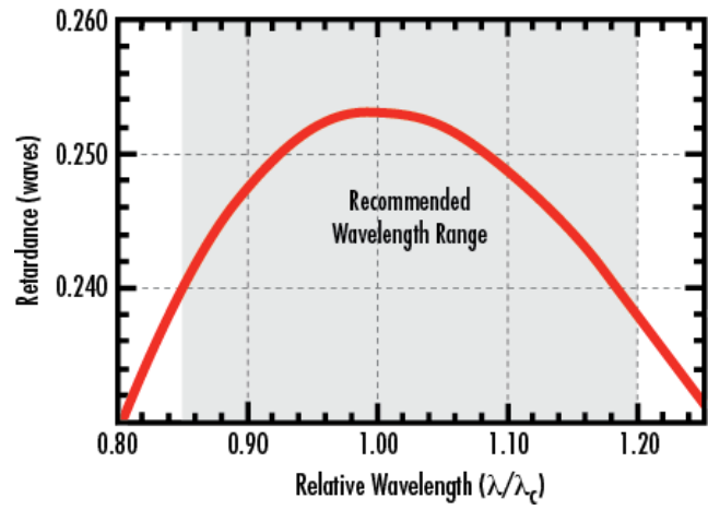
\lambda/4 Precision Achromatic Retarder Performance
