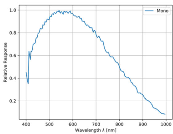
IMX547 Sensor QE Curve
