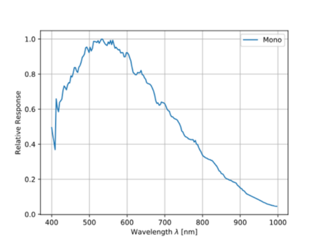
GMX2505 Sensor QE Curve
