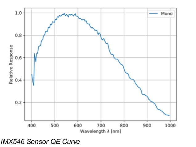
IMX546 Sensor QE Curve
