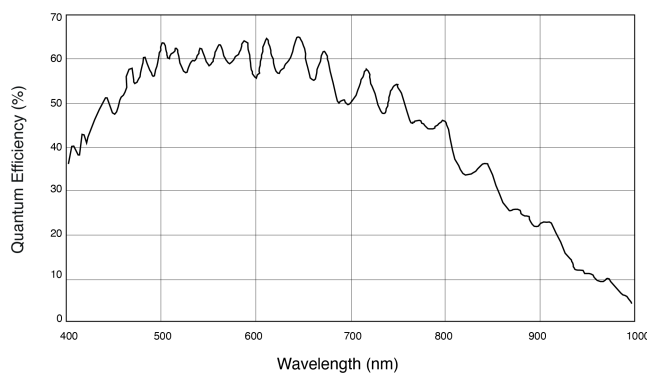
MT9P031 Sensor QE Curve
