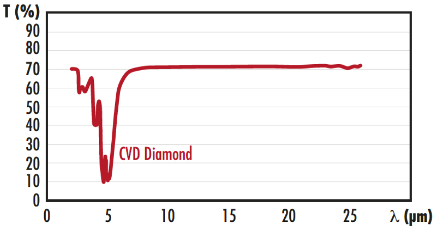
Infrared Windows Transmission
