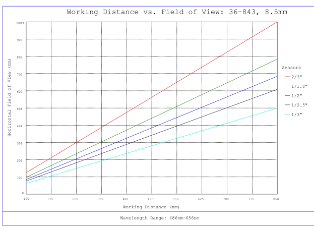
#36-843, 8.5mm, f/8 Cr Series Fixed Focal Length Lens, Working Distance versus Field of View Plot
