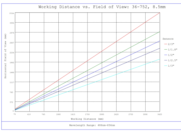
#36-752, 8.5mm f/8, 75mm-∞ Primary WD, HRi Series Fixed Focal Length Lens, Working Distance versus Field of View Plot
