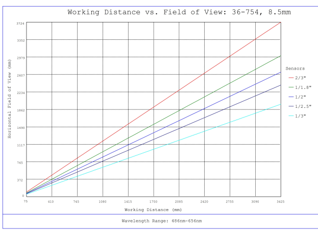
#36-754, 8.5mm f/16, 75mm-∞ Primary WD, HRi Series Fixed Focal Length Lens, Working Distance versus Field of View Plot
