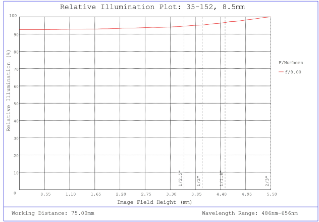
#35-152, 8.5mm, f/8.0, 75mm-∞ Primary WD, HRr Series Fixed Focal Length Lens, Relative Illumination Plot
