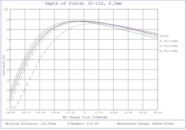
#35-152, 8.5mm, f/8.0, 75mm-∞ Primary WD, HRr Series Fixed Focal Length Lens, Depth of Field Plot, 150mm Working Distance, f8
