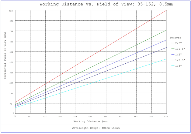
#35-152, 8.5mm, f/8.0, 75mm-∞ Primary WD, HRr Series Fixed Focal Length Lens, Working Distance versus Field of View Plot
