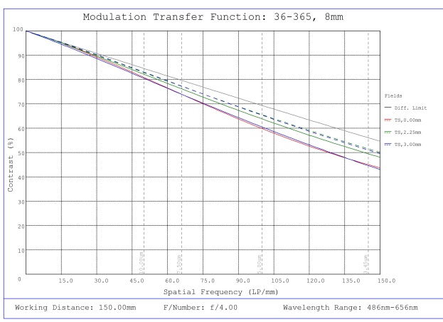
#36-365, 8.0mm FL f/4 Rugged Blue Series M12 Lens, Modulated Transfer Function (MTF) Plot, 150mm Working Distance, f4
