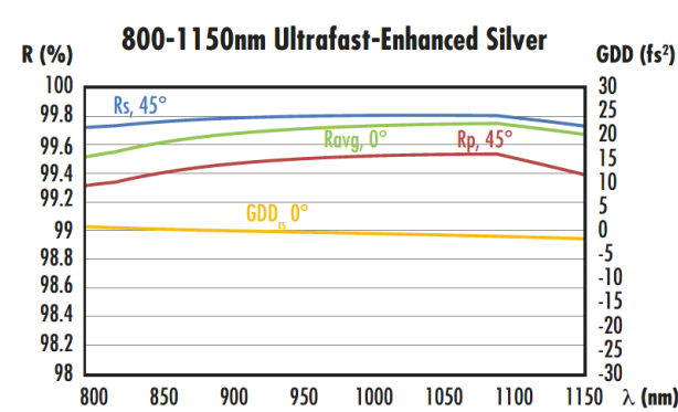
800-1150nm Ultrafast-Enhanced Silver
