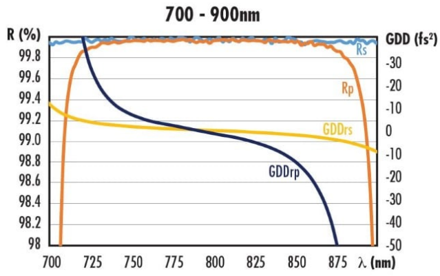
Ultrafast Ti:Sapphire Laser Mirror Reflection Curve
