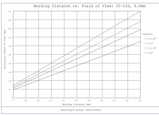
#35-143, 6mm, f/5.6 Cr Series Fixed Focal Length Lens, Working Distance versus Field of View Plot
