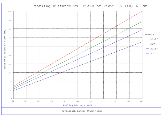
#35-140, 6mm, f/1.8 Cr Series Fixed Focal Length Lens, Working Distance versus Field of View Plot
