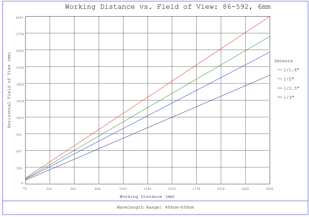
#86-592, 6mm, f/1.8 Ci Series Fixed Focal Length Lens, Working Distance versus Field of View Plot
