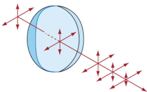
PCX Circular
