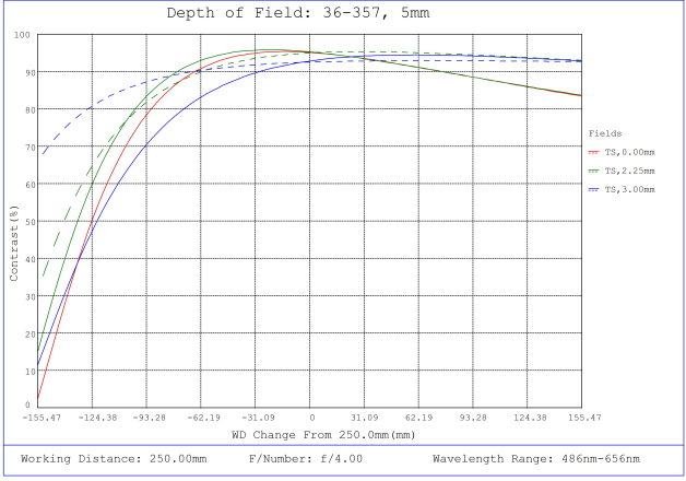
#36-357, 5mm FL f/4, Rugged Blue Series M12 Lens, Depth of Field Plot, 250mm Working Distance, f4
