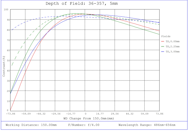
#36-357, 5mm FL f/4, Rugged Blue Series M12 Lens, Depth of Field Plot, 150mm Working Distance, f4
