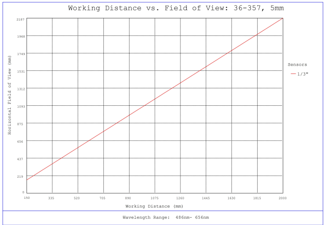
#36-357, 5mm FL f/4, Rugged Blue Series M12 Lens, Working Distance versus Field of View Plot
