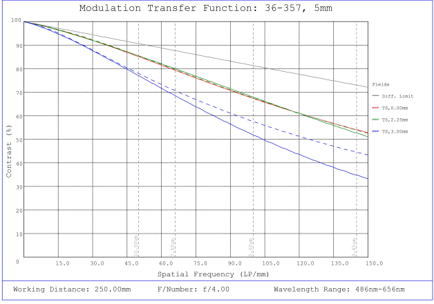
#36-357, 5mm FL f/4, Rugged Blue Series M12 Lens, Modulated Transfer Function (MTF) Plot, 250mm Working Distance, f4
