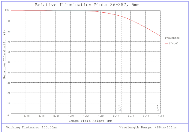
#36-357, 5mm FL f/4, Rugged Blue Series M12 Lens, Relative Illumination Plot
