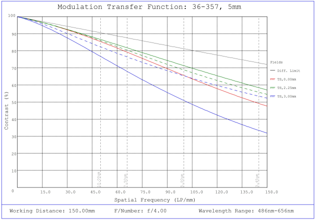
#36-357, 5mm FL f/4, Rugged Blue Series M12 Lens, Modulated Transfer Function (MTF) Plot, 150mm Working Distance, f4
