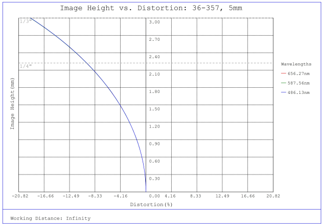
#36-357, 5mm FL f/4, Rugged Blue Series M12 Lens, Distortion Plot
