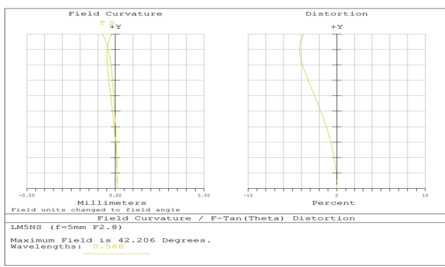
5mm FL, f/2.8, Low Distortion M12 Lens, Distribution Plot
