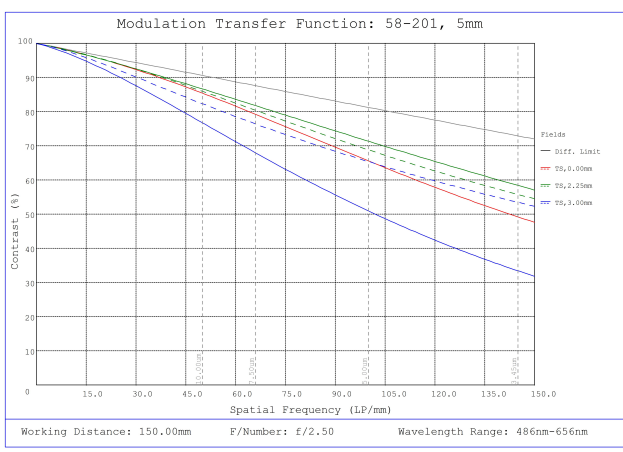
#58-201, 5mm FL f/2.5, Blue Series M12 Lens, Modulated Transfer Function (MTF) Plot, 150mm Working Distance, f2.5
