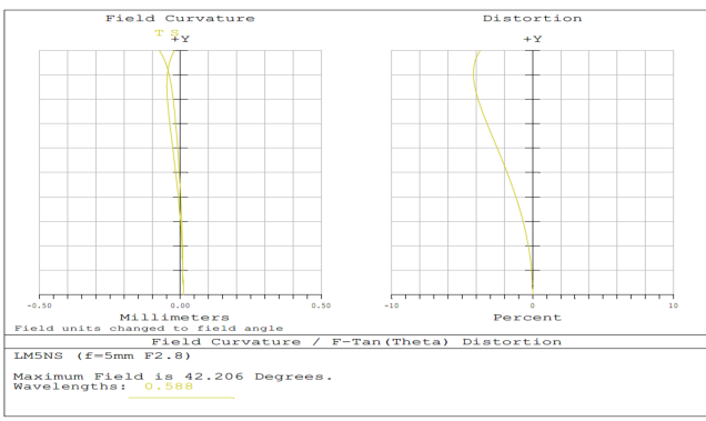
5mm FL, f/2.1, Low Distortion M12 Lens, Distribution Plot
