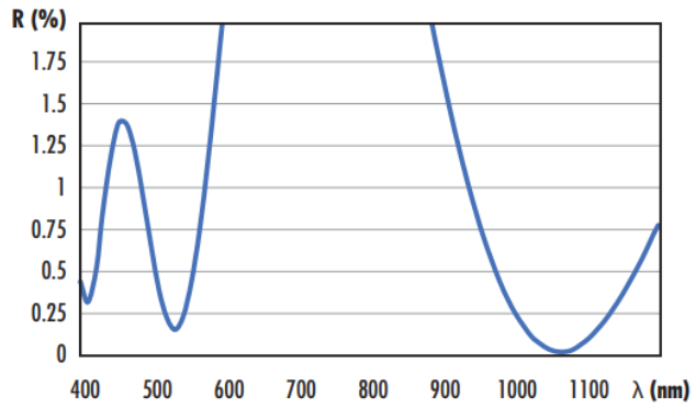
532 & 1064nm Dual-Band AR Coated Laser Window
