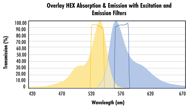
Overlay HEX Absorption and Emission with Excitation and Emission Filters
