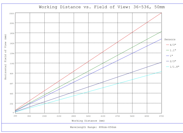
#36-536, 50mm f/8.0, HPr Series Fixed Focal Length Lens, Working Distance versus Field of View Plot
