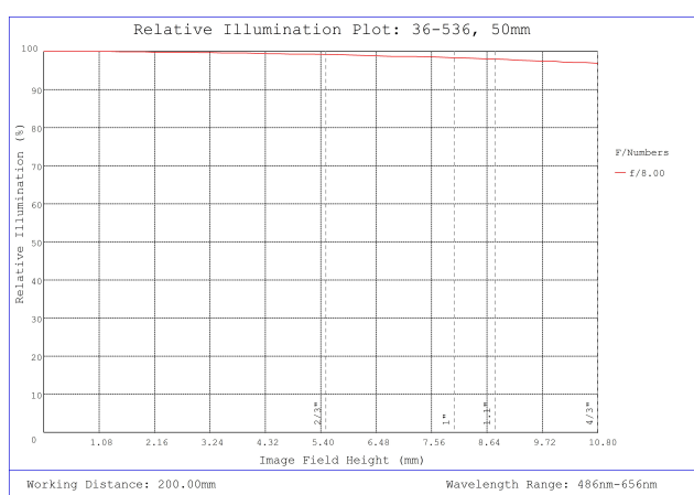
#36-536, 50mm f/8.0, HPi Series Fixed Focal Length Lens, Relative Illumination Plot
