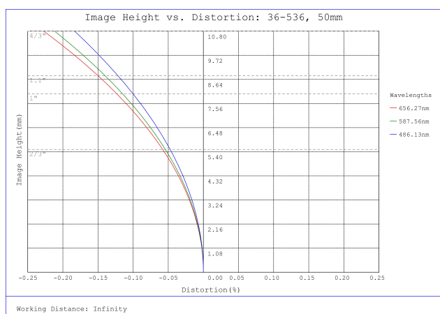
#36-536, 50mm f/8.0, HPi Series Fixed Focal Length Lens, Distortion Plot
