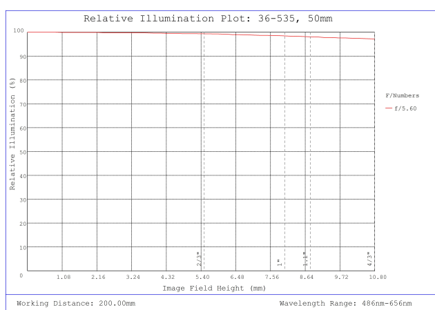
#36-535, 50mm f/5.6, HPi Series Fixed Focal Length Lens, Relative Illumination Plot
