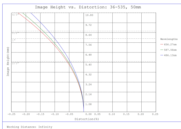
#36-535, 50mm f/5.6, HPi Series Fixed Focal Length Lens, Distortion Plot
