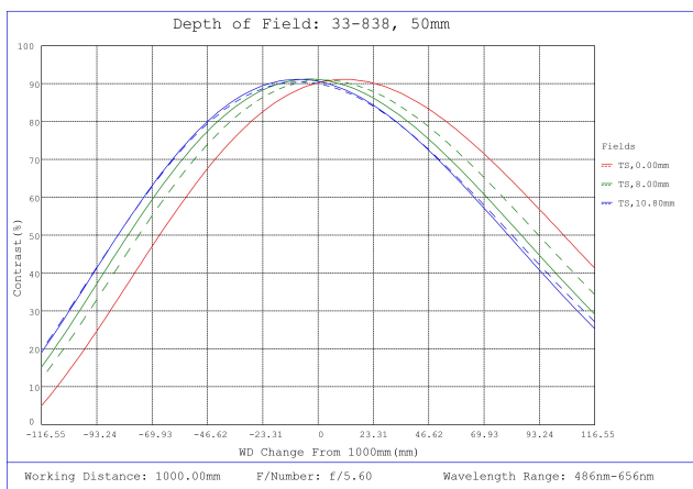
#33-838, 50mm f/5.6, HPI Series Fixed Focal Length Lens, Depth of Field Plot, 1000mm Working Distance, f5.6
