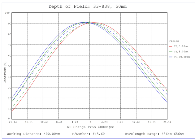
#33-838, 50mm f/5.6, HPI Series Fixed Focal Length Lens, Depth of Field Plot, 400mm Working Distance, f5.6
