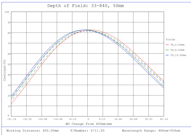
#33-840, 50mm f/11, HPI Series Fixed Focal Length Lens, Depth of Field Plot, 400mm Working Distance, f11
