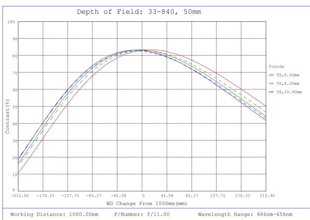
#33-840, 50mm f/11, HPI Series Fixed Focal Length Lens, Depth of Field Plot, 1000mm Working Distance, f11
