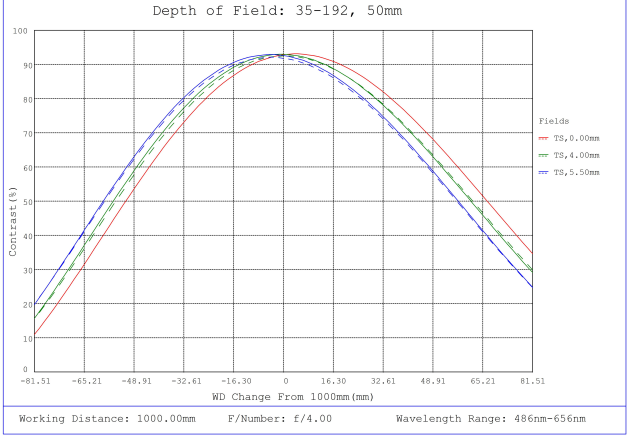
#35-192, 50mm, f/4.0 Cr Series Fixed Focal Length Lens, Depth of Field Plot, 1000mm Working Distance, f4
