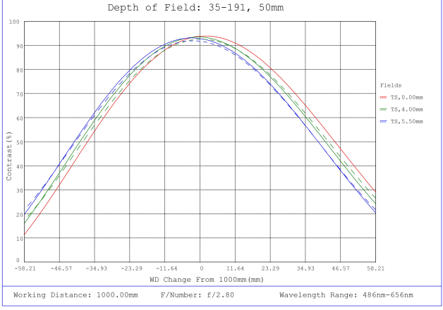
#35-191, 50mm, f/2.8 Cr Series Fixed Focal Length Lens, Depth of Field Plot, 1000mm Working Distance, f2.8
