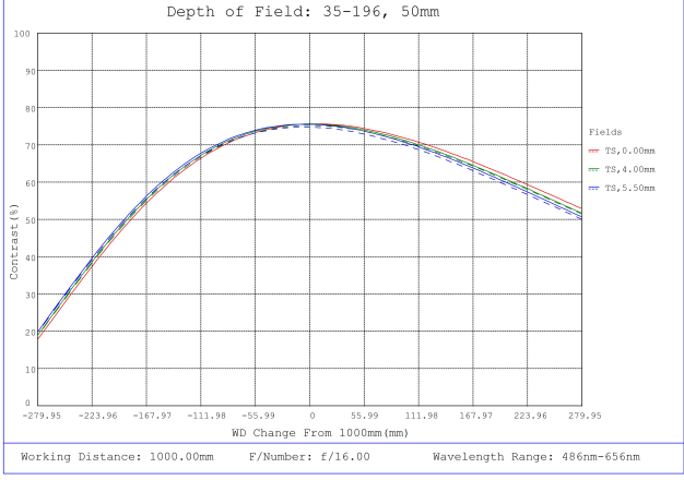
#35-196, 50mm, f/16 Cr Series Fixed Focal Length Lens, Depth of Field Plot, 1000mm Working Distance, f16
