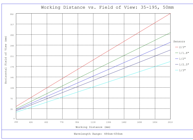
#35-195, 50mm, f/11 Cr Series Fixed Focal Length Lens, Working Distance versus Field of View Plot
