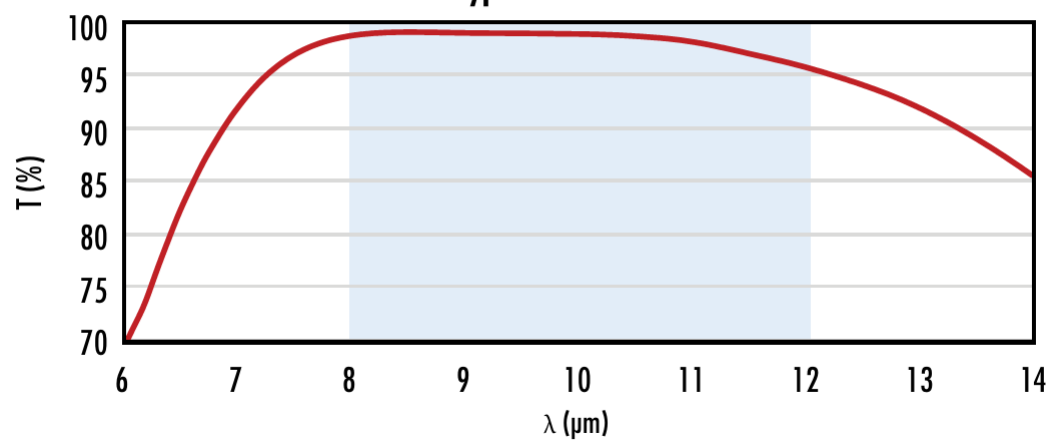
ZnSe with 8-12 \mu\text{m} AR Coating Typical Transmission
