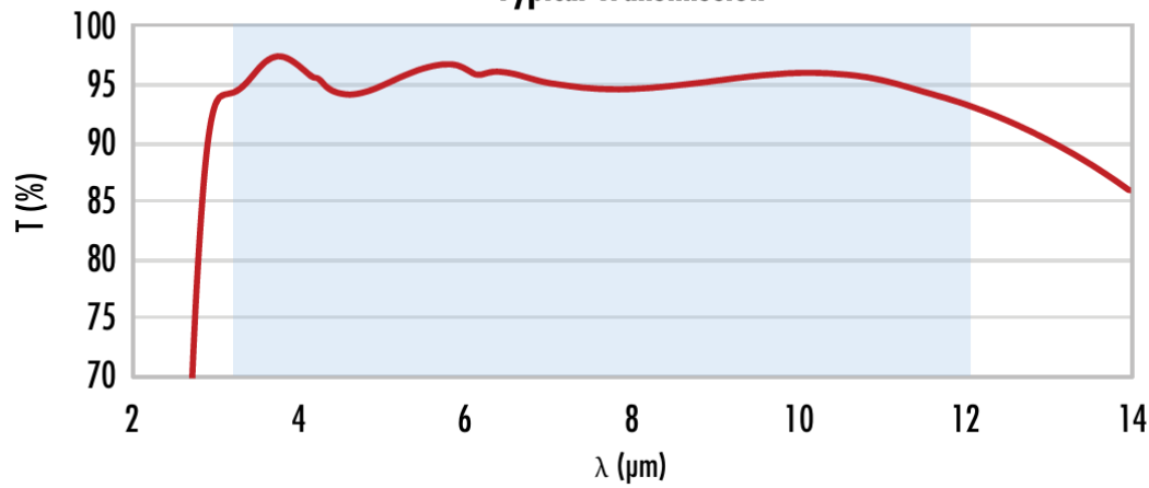
ZnSe with 3-12 \mu\text{m} AR Coating Typical Transmission
