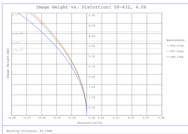
#58-432, 4.0X SilverTL™ Telecentric Lens, Distortion Plot
