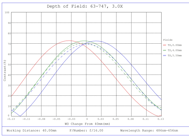
#63-747, 3X, 40mm WD CompactTL™ Telecentric Lens , Depth of Field Plot, 40mm Working Distance, f16
