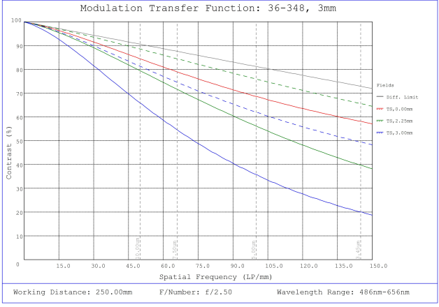
#36-348, 3mm FL f/2.5, Rugged Blue Series M12 Lens, Modulated Transfer Function (MTF) Plot, 250mm Working Distance, f2.5
