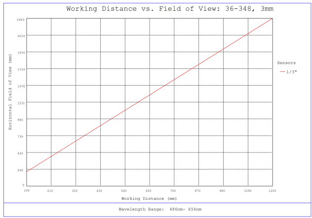
#36-348, 3mm FL f/2.5, Rugged Blue Series M12 Lens, Working Distance versus Field of View Plot
