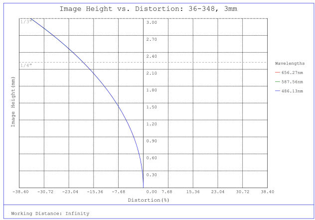
#36-348, 3mm FL f/2.5, Rugged Blue Series M12 Lens, Distortion Plot
