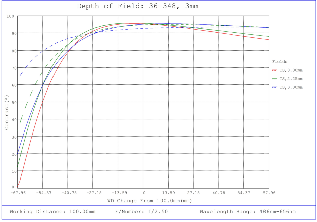
#36-348, 3mm FL f/2.5, Rugged Blue Series M12 Lens, Depth of Field Plot, 100mm Working Distance, f2.5
