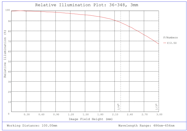
#36-348, 3mm FL f/2.5, Rugged Blue Series M12 Lens, Relative Illumination Plot
