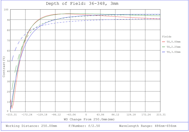
#36-348, 3mm FL f/2.5, Rugged Blue Series M12 Lens, Depth of Field Plot, 250mm Working Distance, f2.5
