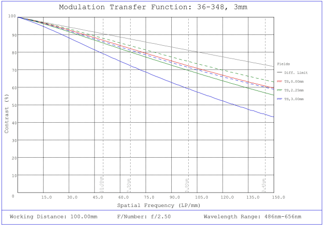
#36-348, 3mm FL f/2.5, Rugged Blue Series M12 Lens, Modulated Transfer Function (MTF) Plot, 100mm Working Distance, f2.5
