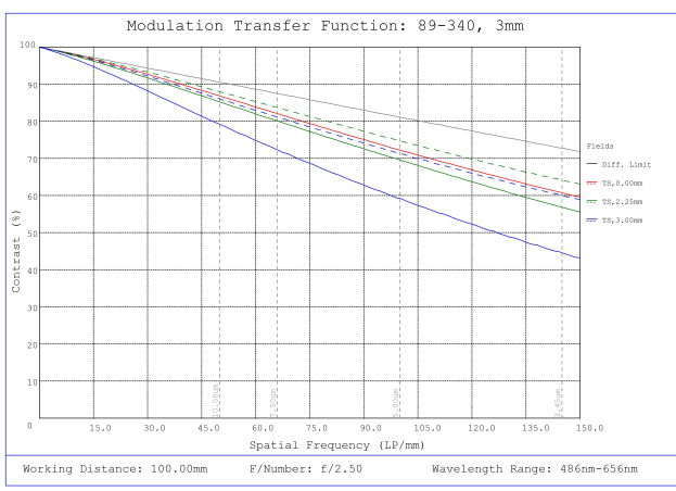
#89-340, 3mm FL f/2.5, Blue Series M12 Lens, Modulated Transfer Function (MTF) Plot, 100mm Working Distance, f2.5
