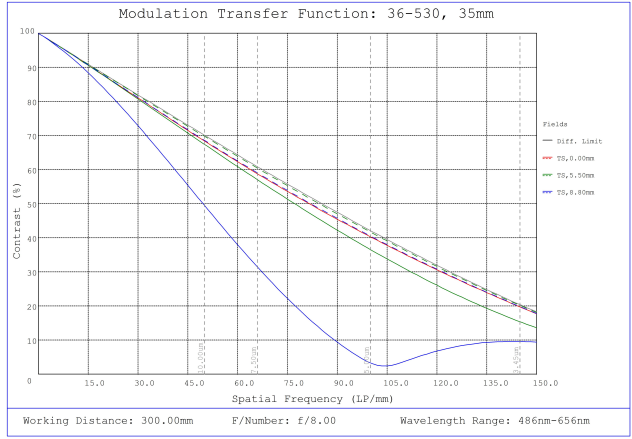
#36-530, 35mm f/8.0, HPr Series Fixed Focal Length Lens, Modulated Transfer Function (MTF) Plot, 300mm Working Distance, f8
