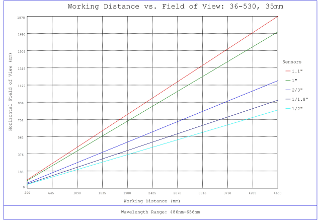
#36-530, 35mm f/8.0, HPr Series Fixed Focal Length Lens, Working Distance versus Field of View Plot
