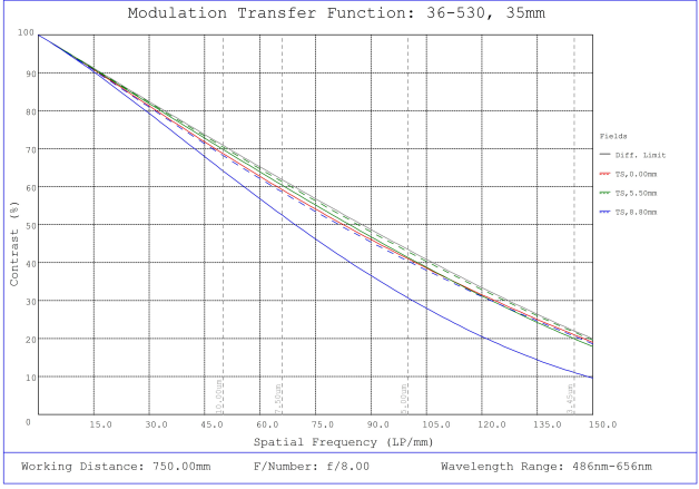
#36-530, 35mm f/8.0, HPr Series Fixed Focal Length Lens, Modulated Transfer Function (MTF) Plot, 750mm Working Distance, f8
