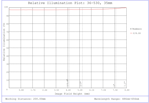
#36-530, 35mm f/8.0, HPr Series Fixed Focal Length Lens, Relative Illumination Plot
