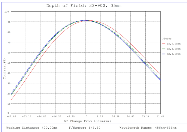
#33-900, 35mm f/5.6, UCI Series Fixed Focal Length Lens, Depth of Field Plot, 400mm Working Distance, f5.6
