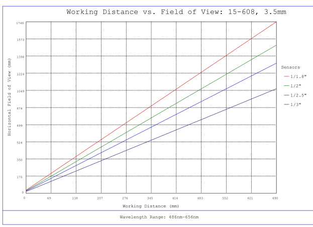
#15-608, 3.5mm f/2.8 Sealed Cw Series Fixed Focal Length Lens, Working Distance versus Field of View Plot
