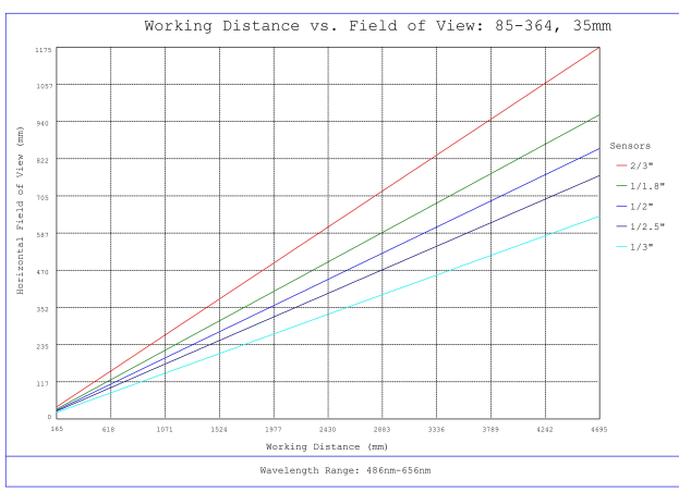
#85-364, 35mm, f/2.8 Ci Series Fixed Focal Length Lens, Working Distance versus Field of View Plot
